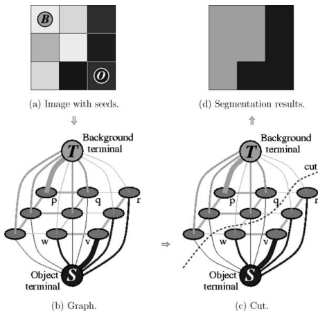
Figure 13: Minimum graph cut segmentation of a 3x3 image. Image from [1].
