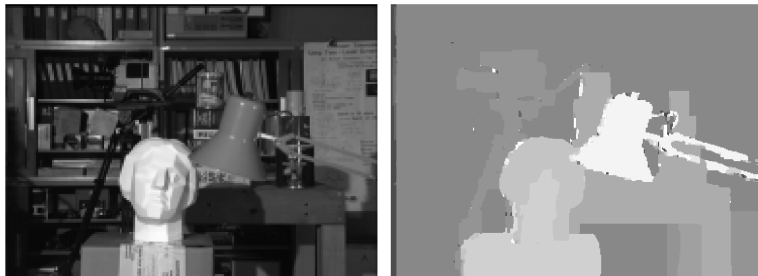
Figure 19: Left: One image in a stereo pair. Right: Depth estimated with graph cuts.
